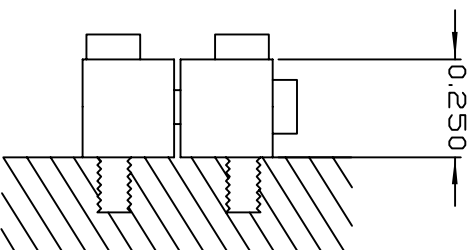
WALL MOUNTING
